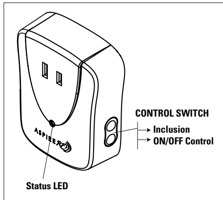
Figure 1. RFAPM – Application Diagram
