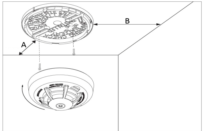
Figure 2 Mounting the Alarm
