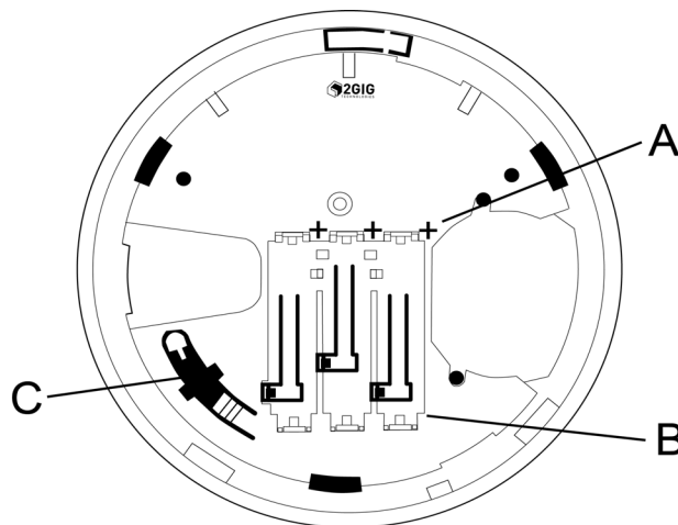
Figure 5 Wireless Smoke & Heat Alarm—Battery Compartment
