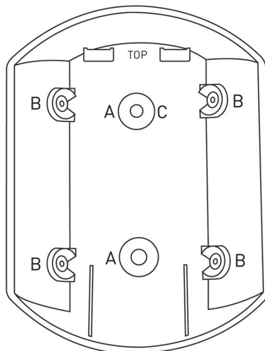
Figure 4 PIR Backplate—Direct-to-Wall Mounting Guides
